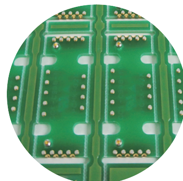
With different types of pin terminals inserted
